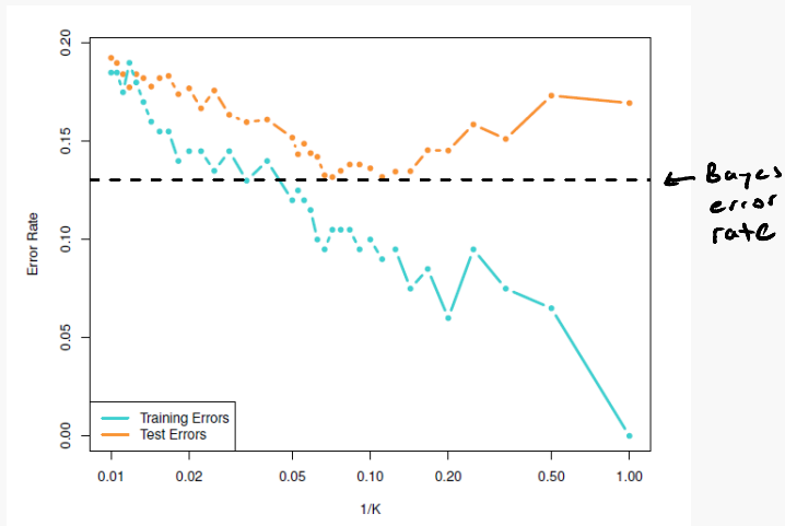
Figure 14: Image by James et al. (2021). The KNN training error rate (in blue) and test error rate (in orange) and the Bayes error rate (in black). The jumpiness of the curves is due to the small size of the training data set.
