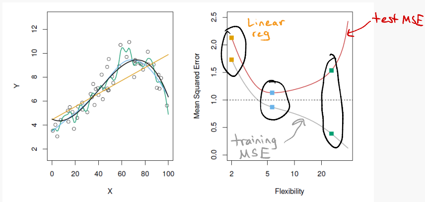
Figure 10: Image by James et al. (2021). Left: Data simulated from f (in black). Three estimates for f : Linear regression (in orange), and two smoothing splines (in blue and green). Right: Training MSE (in grey), test MSE (in red), and minimum possible test MSE over all methods (dashed line). The squares represent the three fits from the left panel.
